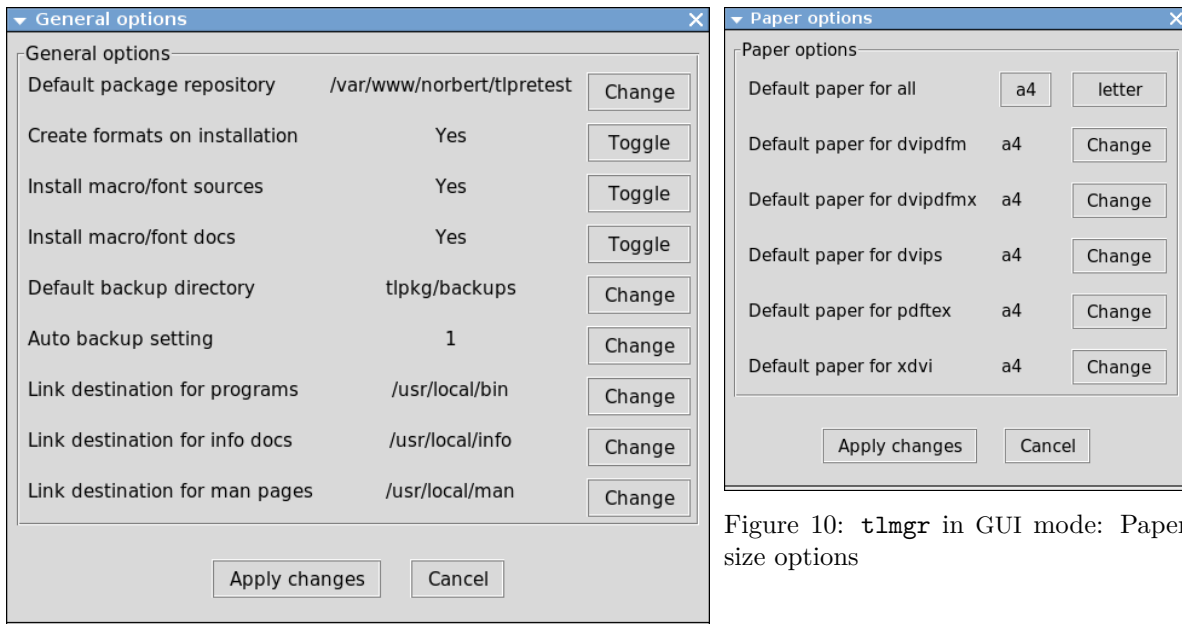
Figure 9: tlmgr in GUI mode: General options
